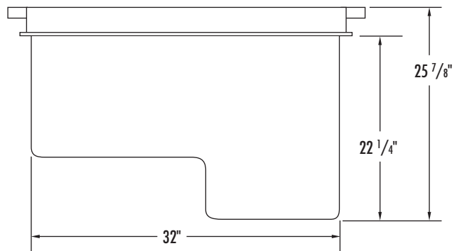
FRONT (Seat Closed) Right Hand Shown
